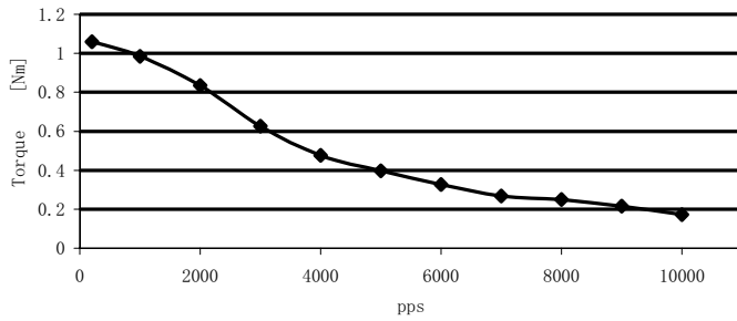
FL57STH76-3006MA
