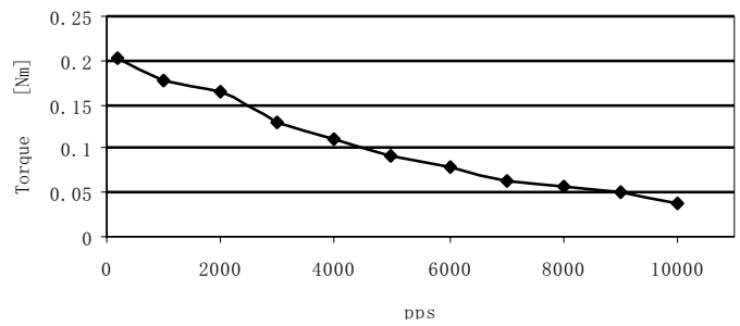
FL42STH33-1334MA
