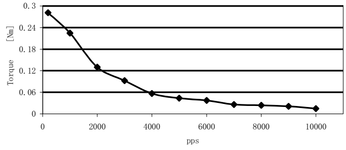
FL42STH33-1334A
