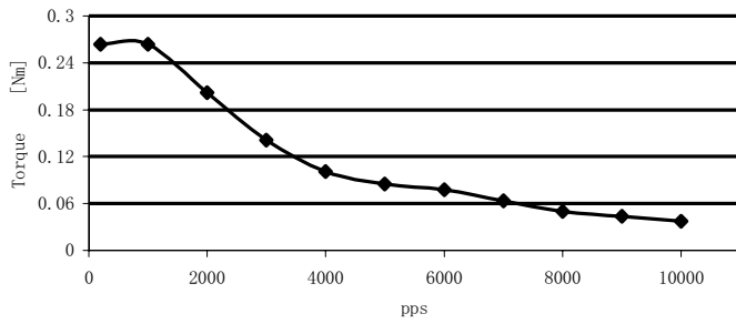
FL42STH47-0406MA
