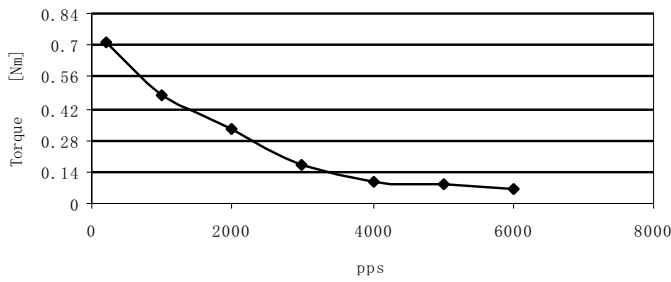
FL57ST76-0686A
