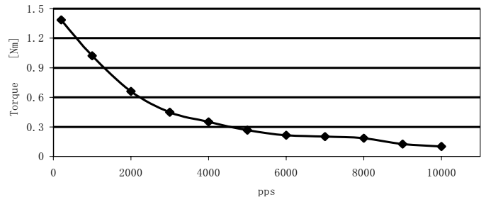
FL57STH76-2804MA
