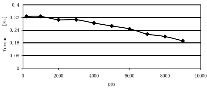
FL57STH41-3006MA
