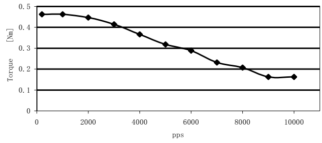
FL42STH47-1684A
