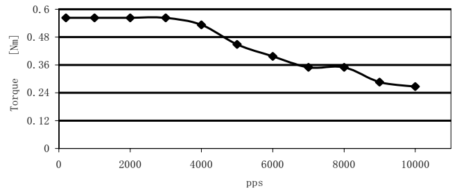
FL57STH51-2006A
