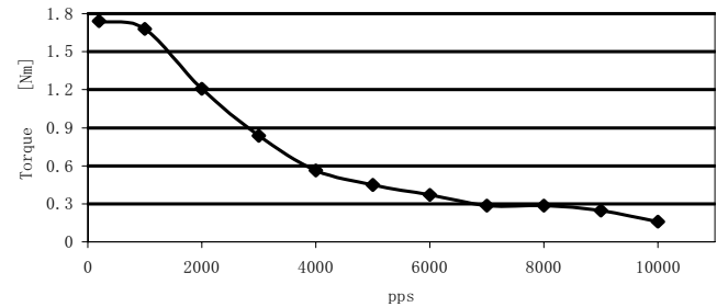
FL57STH76-2804A
