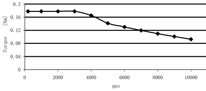
FL42STH33-0316A
