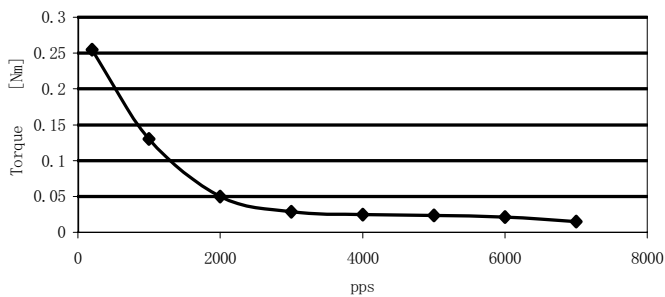
FL39ST44-0304A
