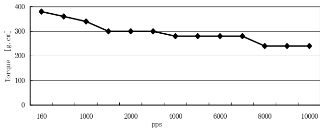
FL28STH32-0956A VM:24VDC;0.95A/Phase() Driver:M415B, half step
