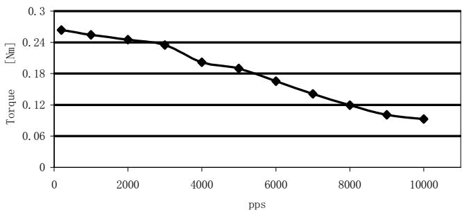
FL42STH38-1206A
