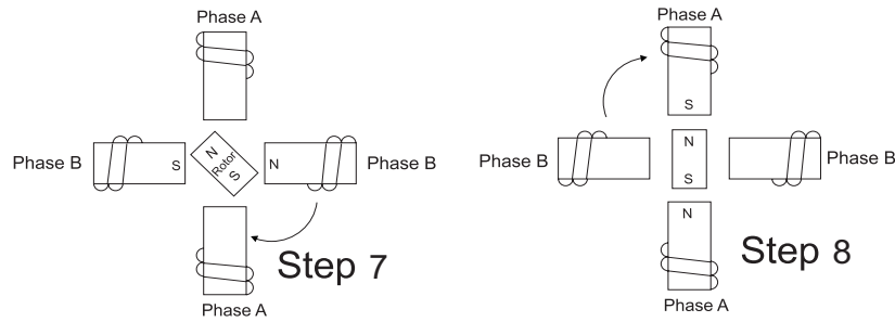
Figure 3. Half-stepping-90° step angle is reduced to 45° with half-stepping.
